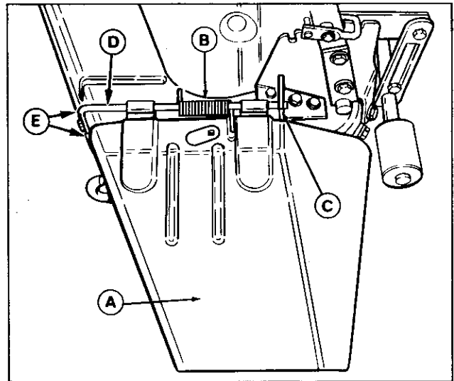
Figure 1. 48" Mower
